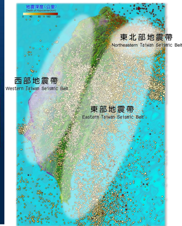
Seismic Belts in Taiwan
